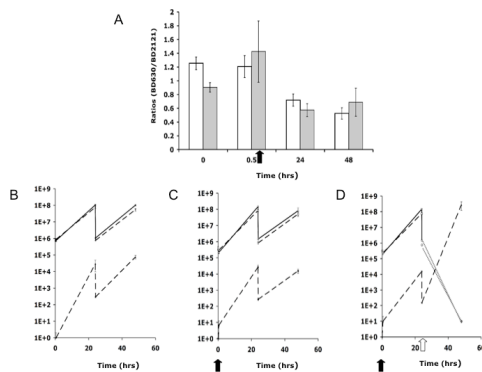
Fig. 6. Competitions between BD630 and BD2121 under conditions where penicillin G pulses are insufficient to provide an advantage to com + over com - cells. A) Ratios of BD630-1/BD2121 in pair-wise competitions with (grey bars) and without (white bars) a single 0.5-hour pulse of penicillin G. B, C and D, changes in the density of com + (top broken line) and com - (top solid line) parental strains and com + transformants (ascending broken line). B – No penicillin pulse, C- 0.5-hour penicillin pulse, D – 0.5-hour penicillin pulse followed by the addition of both kanamycin (25 mg/L) and chloramphenicol (5 mg/L). Means and 95% confidence intervals of the replicas transferred to fresh medium at 24 hours. The solid block arrow indicates penicillin pulse; the open block arrow indicates the introduction of kanamycin and chloramphenicol. Note that we were unable to detect parental com + or com - cells at 48 hours and 24 hours after antibiotics were added to select for transformants.
