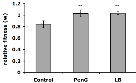
Fig. 4. Estimated fitness, w , of com^+ (BD630) in pairwise competition with com^- (BD2121). Control; Competence medium w = 0.84 \pm 0.06 (mean and 95% confidence interval for 9 independent replicas). PenG; 2 hour pulse of penicillin G, w = 1.04 \pm 0.06 . LB; w = 1.03 \pm 0.02 ) ** p < 0.001 Pen G vs. control and LB vs. control.
