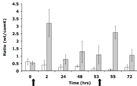
Fig. 5. Ratios of BD630/BD2121 during the course of a serial transfer experiment. Block arrows indicate the addition of 100 mg/L penicillin G followed by the addition of penicillinase 2 hours later. Unshaded bars are untreated controls. Shaded bars are the cultures with penicillin pulsing. Means of three parallel experiments \pm 95% confidence intervals.
